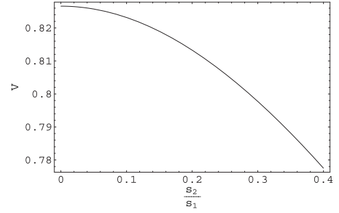
Fig. 5. The visibility of the interference pattern produced by an ultracold cloud released from an optical superlattice as a function of s_2/s_1 with U_{eff}/J_0 = 40 and n_0 = 3 . As the strength of the secondary lattices increases, the visibility worsens since the system gradually goes deeper into the Mott insulator regime and a corresponding gradual loss of long range coherence. A finite visibility even for a Mott-insulator is due to short range coherence since the system consists of a small admixture of particle-hole pairs on top of a perfect Mott-insulator. A loss of visibility in the superlattice naturally means that there is loss of particle-hole pairs.
